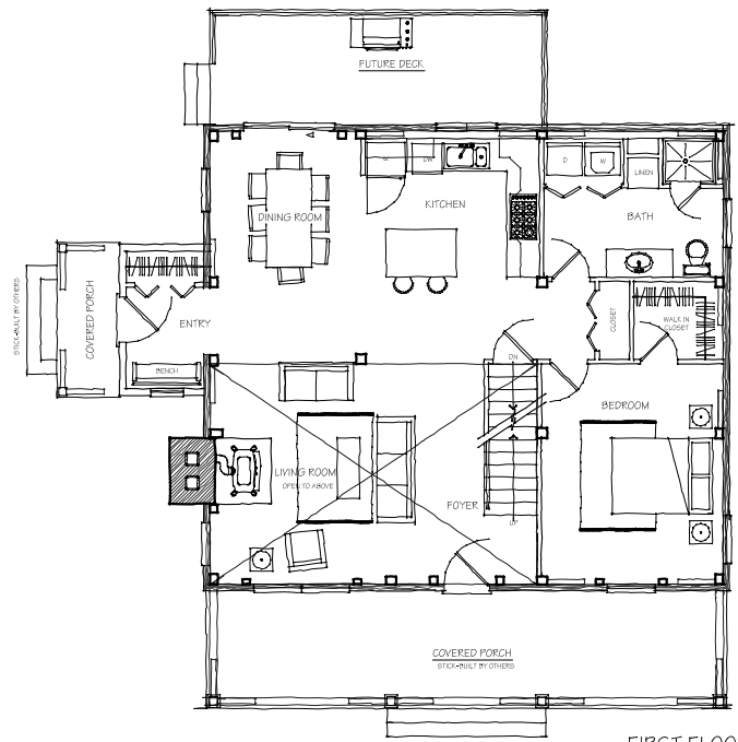
FIRST FLOOR PLAN FINISHED SPACE = 1075 S.F.
