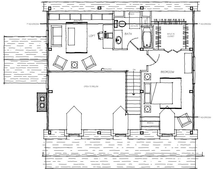
SECOND FLOOR PLAN FINISHED SPACE = 675 S.F.
