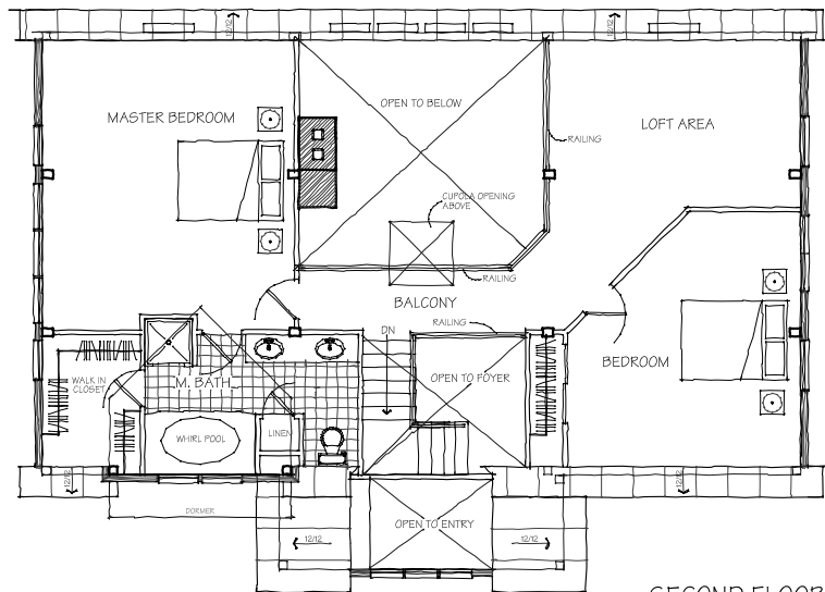
SECOND FLOOR PLAN 2nd FLOOR PLAN = 1000 s.f.
