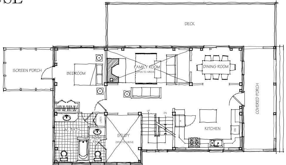
FIRST FLOOR PLAN 1st FLOOR PLAN = 1056 s.f.
